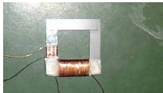
Fig.1 Tested Yoke and Exciting Coil
