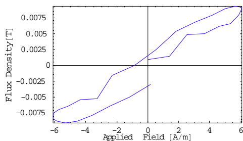
Fig.5 Averaged Magnetization Characteristic Curve
