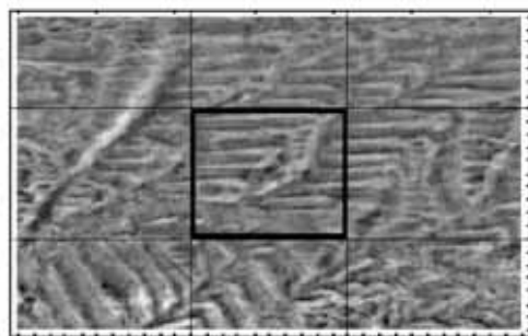
Fig.6 Sample Area for Local Magnetization Characteristic Extraction
