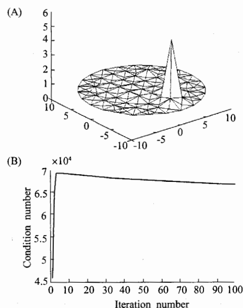
Fig.2 (A)The conductivities distribution in the reconstructed field; (B)Relationship of number of iterations and condition number of reconstruction matrix
